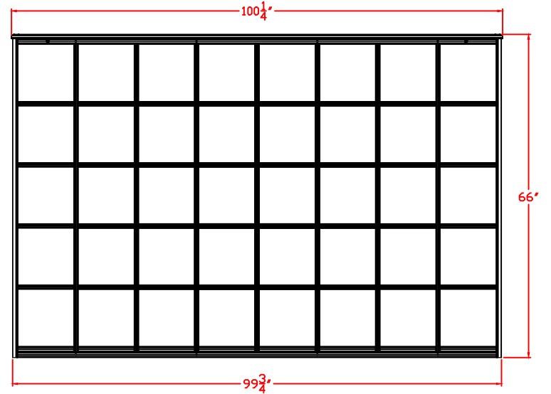
REAR VIEW
